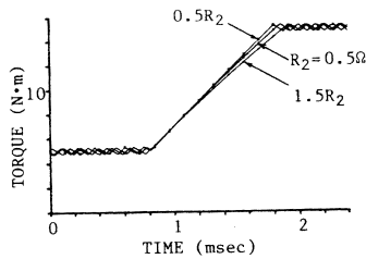
Fig. 11. Torque step response for variations of R_2 .
