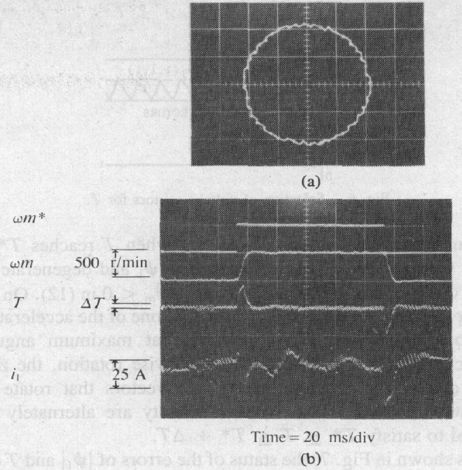
Fig. 9. Experimental results. (a) Locus of \psi_1 at 600 r/min. (b) Velocity step response.
